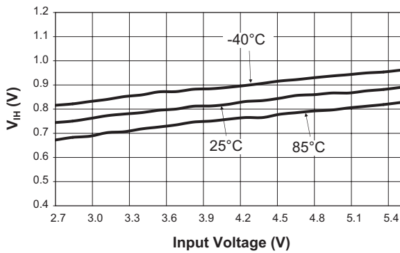
Enable Input High Threshold vs. Input Voltage
